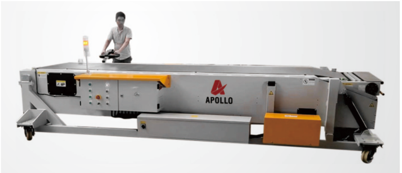
APOLLO motorized movement telescopic belt conveyor One operator can move machine easily
